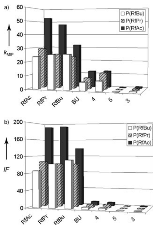
Figure 2. a) Retention factors ( k ) and b) imprinting factors ( IF ) obtained in the chromatographic evaluation of the riboflavin tetraester imprinted polymers (P(RfAc), P(RfPr), P(RfBu)) and a control, non-imprinted, polymer (P(N)) using acetonitrile/acetic acid (99/1 v/v) as the mobile phase. k and IF are defined as follows: k = (t - t_0)/t_0 ; IF = k_{MIP}/k_{NIP} ; where t = retention time of the solute; t_0 = retention time of a nonretained void marker; k_{MIP} ( k_{NIP} ) = retention factors for a given solute using the imprinted (or non-imprinted) polymer as stationary phase.
