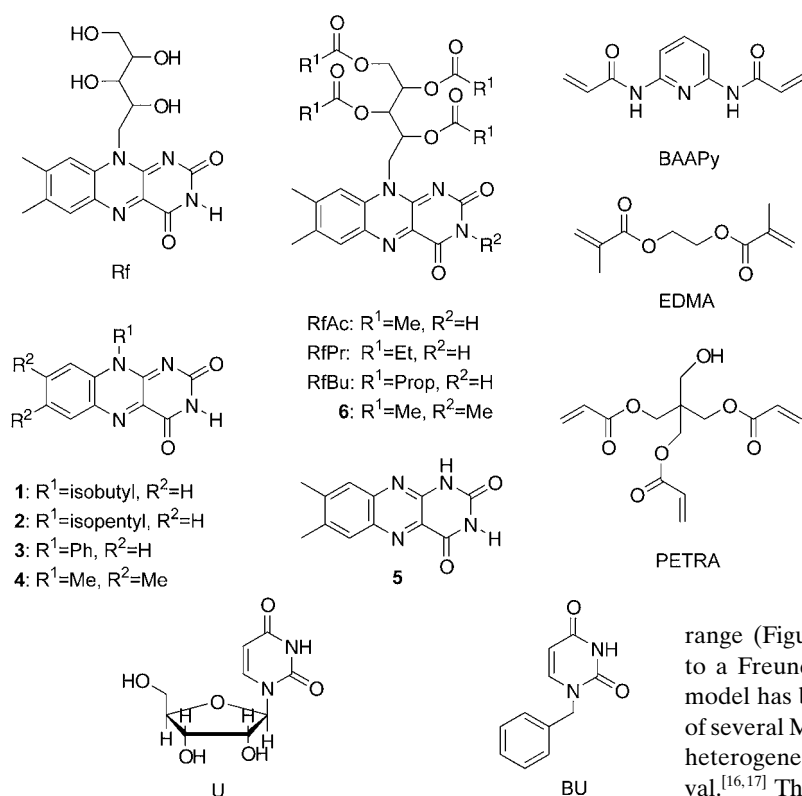
Scheme 1. The monomers and templates investigated in the study.
