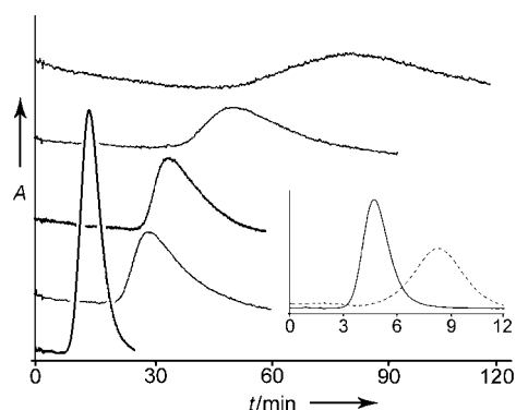
Figure 4. Elution profiles of riboflavin (10 \mu l of a 1 mM solution) injected on columns packed with from bottom to top (main figure): P1, P(RfBu), P(RfPr), P(RfAc), and P(RfAc)'. The inset shows the elution profiles of riboflavin on columns packed with P(N) (dashed line) and P(N)' (solid line). Mobile phase = water/acetonitrile/ethanol (85.5/10/4.5 v/v/v).
