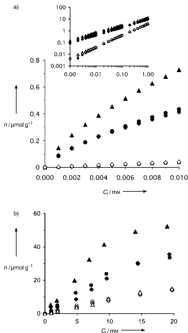
Figure 3. Binding isotherms of riboflavin tetraesters (RfAc: triangles, RfPr: circles, RfBu: diamonds) on their respective complementary polymers (P(RfAc), P(RfPr), P(RfBu): filled symbols) and on a control non-imprinted polymer (P(N); open symbols) as determined a) by frontal analysis using the staircase method or b) by a batch partitioning experiment in acetonitrile/acetic acid (99/1 v/v). In (b) the polymers (10 mg) were equilibrated for 24 h with solutions (0.5 mL) containing different concentrations of the riboflavin tetraesters.
