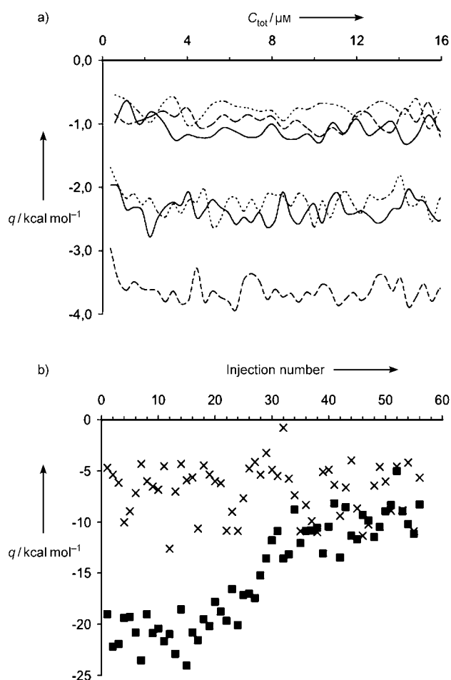
Figure 5. ITC titration profiles showing in a) the energy released ( q ) versus the total concentration of the titrant in the cell ( C_{\text{tot}} ) for the titration of P(RfAc)' (dashed lines), P(N)' (solid lines), or blank (dotted lines) with Rf (lower three profiles) or U (upper three profiles) in water/ethanol/formic acid: 90.6/4.7/4.7 (v/v/v), and b) the energy released versus the injection number for the titration of solutions of Rf (■) or U (X) (1 \mu M in 50 mM aqueous sodium phosphate buffer pH 7) by RfBP.
